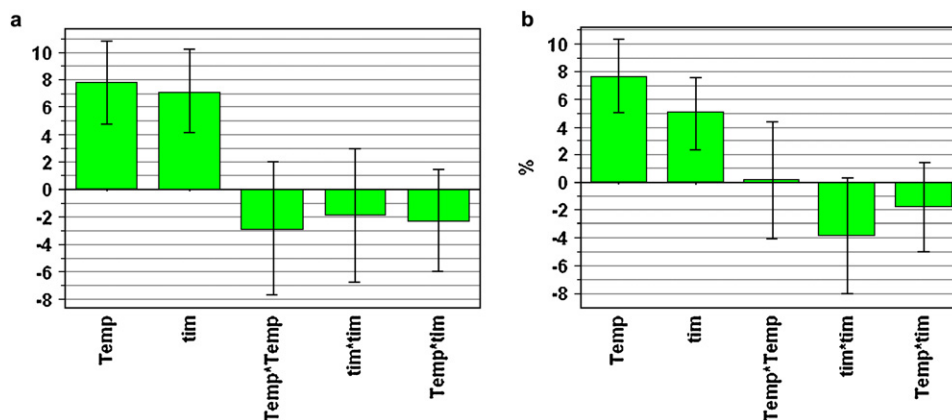
Figure 2. Coefficient plot for temperature–time effect screening for (a) conversion and (b) purity. Each plot contains the terms used in the statistical model. Positive bars indicate a positive impact of the term on the measured response. Negative bars indicate a negative effect. The significance of each term in the model is determined by the size of the bar relative to the error bar. Non-significant terms are small and have an error bar, which spans the axis.
