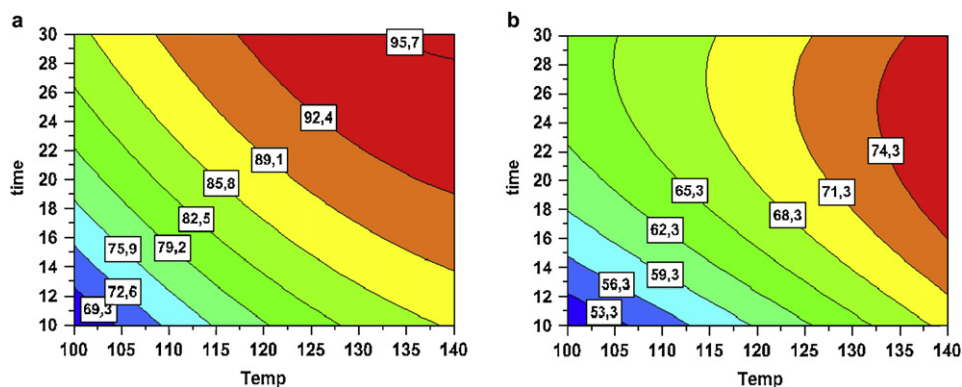
Figure 3. Response surfaces for (a) conversion and (b) purity in dependence of temperature and time. Each contour line indicates a level of the response, e.g., conversion for a given combination of the variables, in this case temperature and time. Blue areas indicate a low response and red areas indicate a high response, thus the optimal regions are red in these plots. Curvature of the lines indicates that the response is non-linear with respect to one or both of the factors. The purity response is strongly curved on the time axis, which is consistent with the significant time \times time term in the model.
