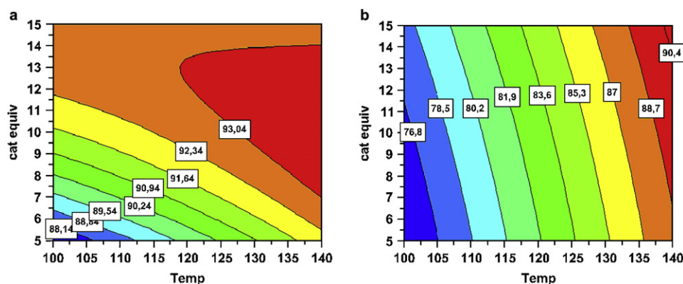
Figure 5. Response surfaces for (a) conversion and (b) purity in dependence of temperature and catalyst concentration.
