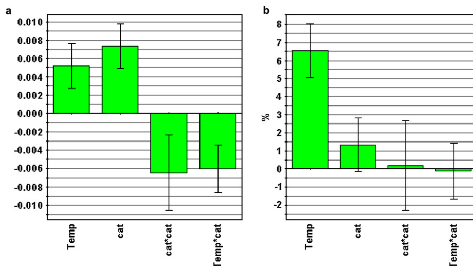
Figure 4. Coefficient plot for temperature–catalyst amount effect screening: for (a) conversion and (b) purity. Each plot contains the terms used in the statistical model. Positive bars indicate a positive impact of the term on the measured response. Negative bars indicate a negative effect. The significance of each term in the model is determined by the size of the bar relative to the error bar. Non-significant terms are small and have an error bar, which spans the axis.
