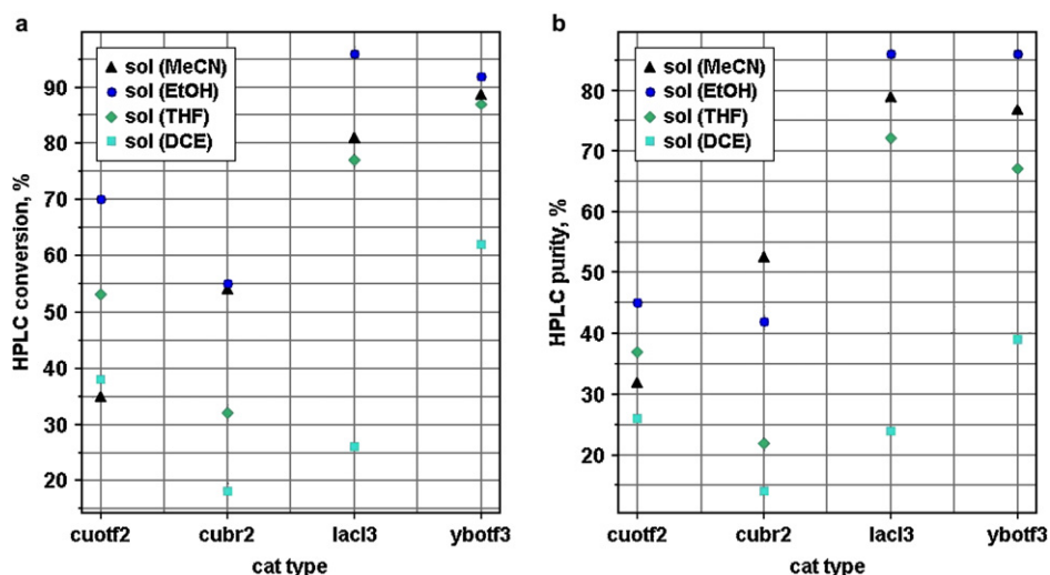
Figure 1. Interaction effects plot of the catalyst/solvent screening for the optimized synthesis of monastrol for (a) conversion and (b) purity. This type of plot enables the effect of both solvent and catalyst to be visualized simultaneously. Clearly the result in terms of conversion and purity is highly dependent on both the choice of solvent and catalyst.
