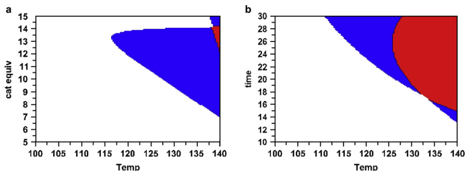
Figure 6. Sweet-spot prediction plots for (a) temperature versus catalyst amount (the set desired values for conversion are in the range 93–95% and 90–100% for purity), and (b) temperature versus time (the set desired values for conversion are in the range 90–96% and 72–80% for purity). Areas in red meet both given criteria, areas in blue meet one of the criteria and in the white area no criteria is met.
